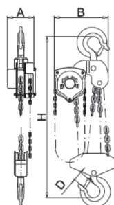
WLL 10t
