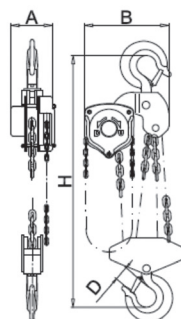
WLL 10t
