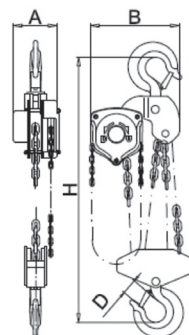
WLL 10t
