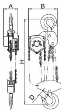
WLL 10t
