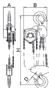
WLL 10t
