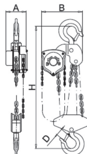
WLL 10t
