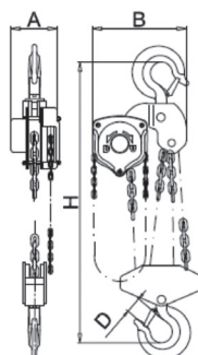
WLL 10t
