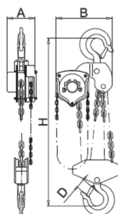
WLL 10t
