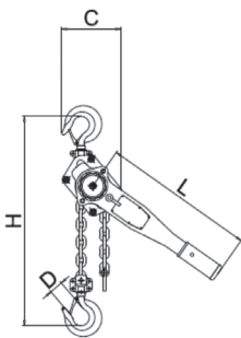
WLL 0.75 t - 3 t
