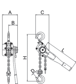
WLL 0.75 t - 3 t
