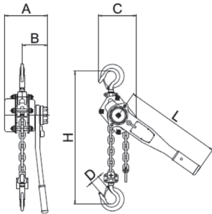
WLL 0.75 t - 3 t
