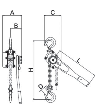
WLL 0.75 t - 3 t
